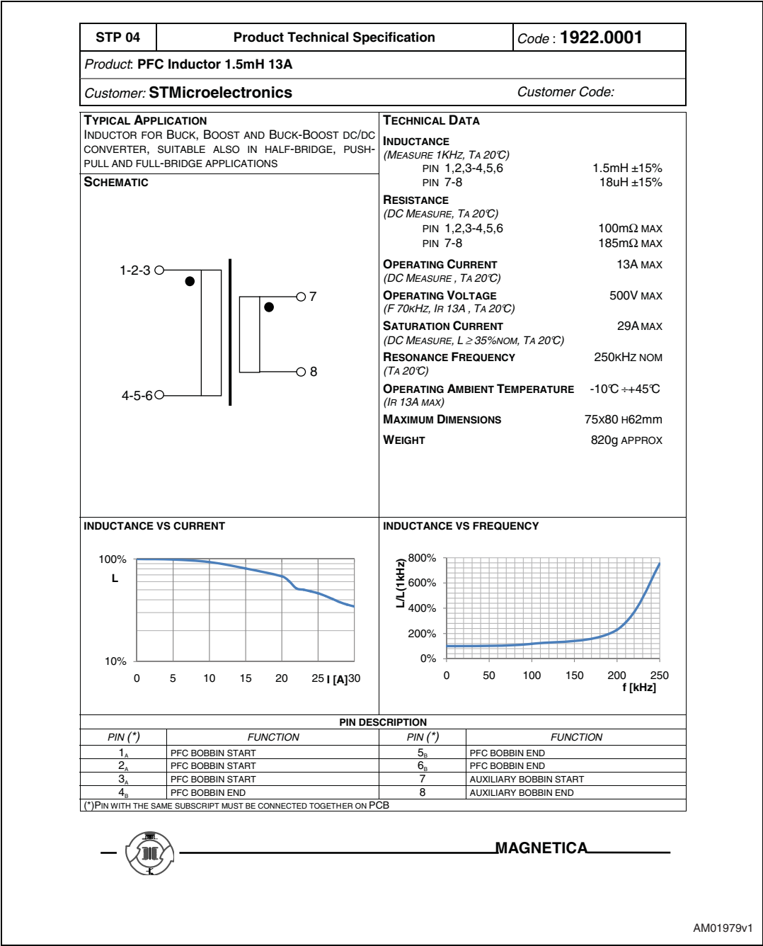
Figure 9. Boost inductor with auxiliary winding, T1 (MAGNETICA 1922.0001) technical sheet
